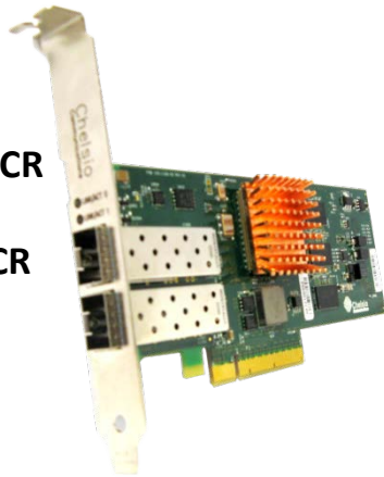
T4 Unified Wire Adapters
